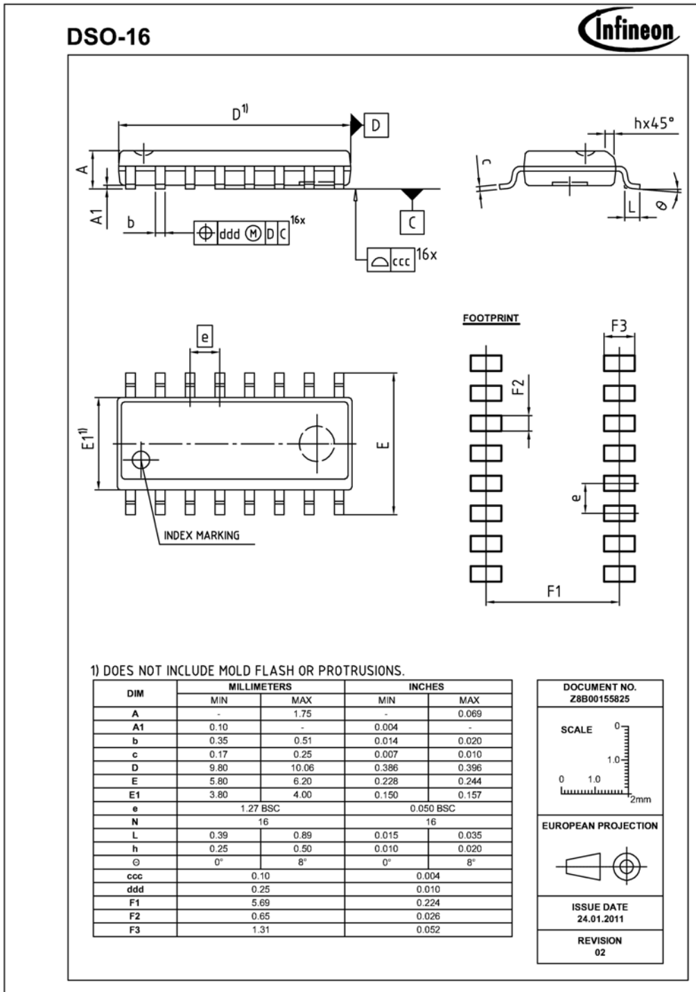
Figure 40 Package Outline with Creepage Distance
