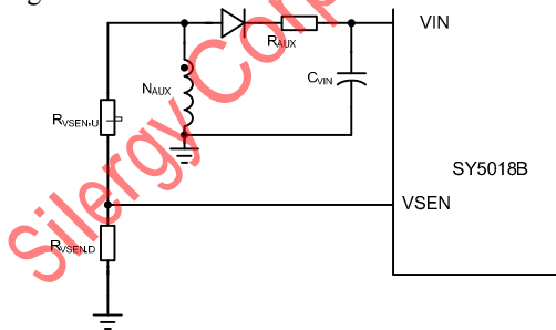
Fig.5 VSEN pin connection
