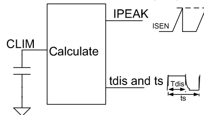
Fig.7 Current sense
