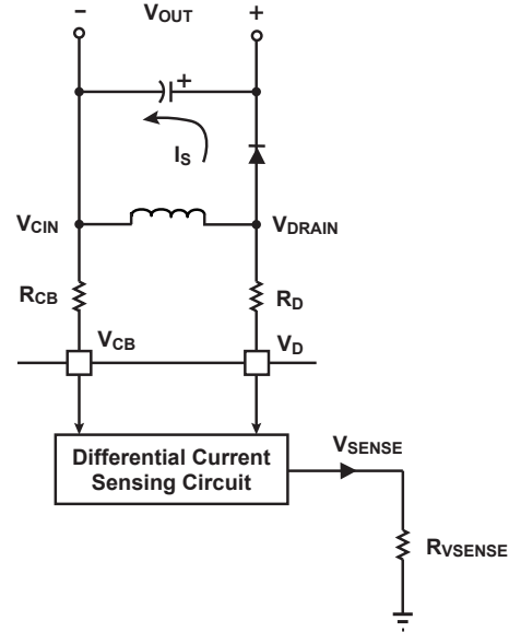
Figure 9.11 : V SENSE Circuit Inside iW3688
