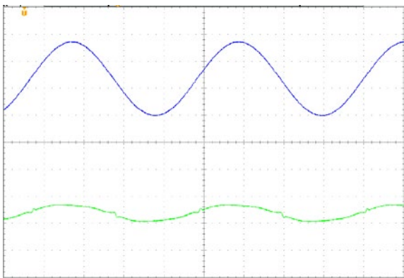
Figure 10.5 : No Dimmer
