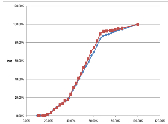
Figure 10.6 : Dimming Curve
