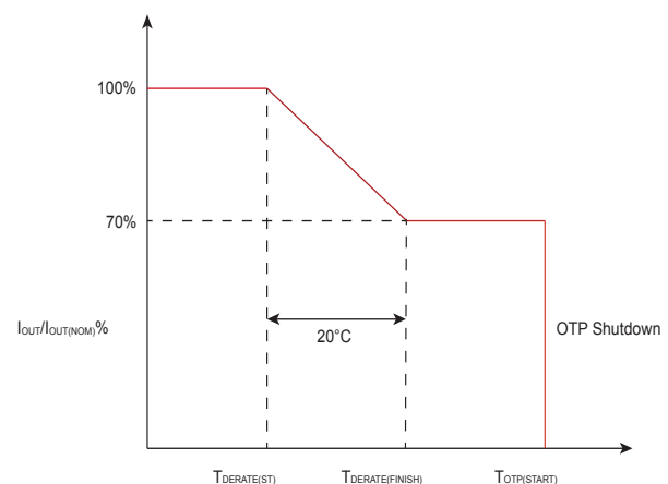
Figure 9.12 : Temperature DeRating and OTP
